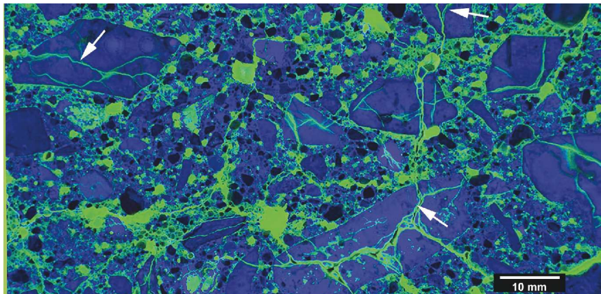
Ultraviolet light photograph of polished slab from a concrete core affected by alkali-silica reaction. The core was impregnated with a fluorescent epoxy. The yellow-green areas are filled with the epoxy. The white arrows indicate examples of cracks.
